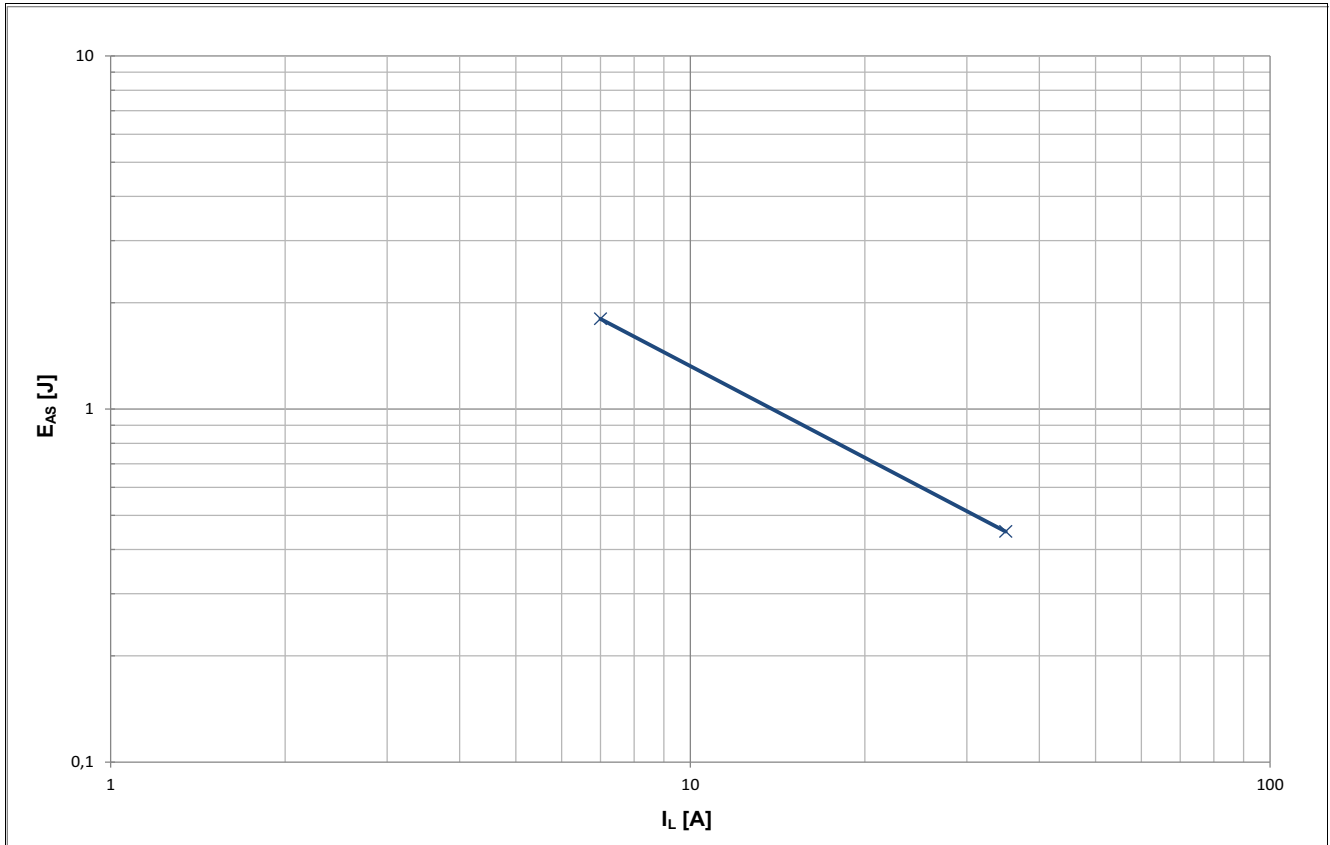
Figure 14 Maximum Energy capability for single pulse E_{AS} = f(I_L) , T_{j(0)} = 150\text{ °C} , V_{BAT} = 28V , V_{IN} = 10V
