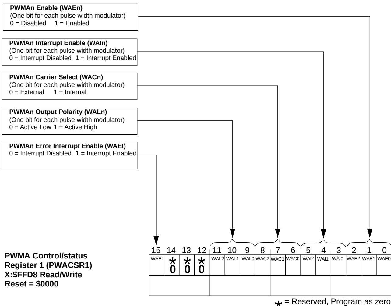
Figure B-40 PWMA Control/status Register 1 (PWACSR1)
