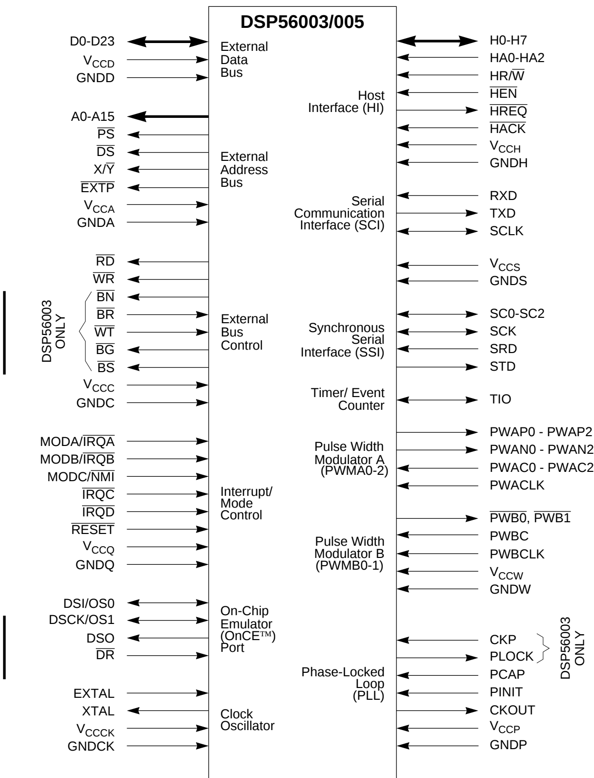
Figure C-2 (2-1) DSP56003/005 Signals
