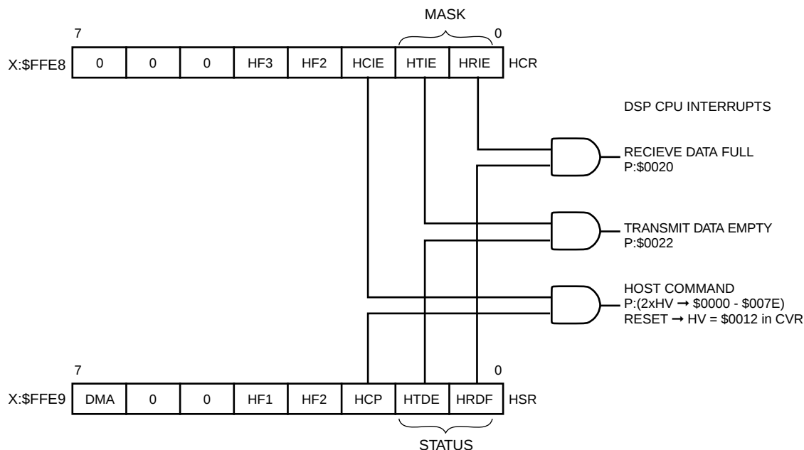
Figure 5-11 HSR-HCR Operation
