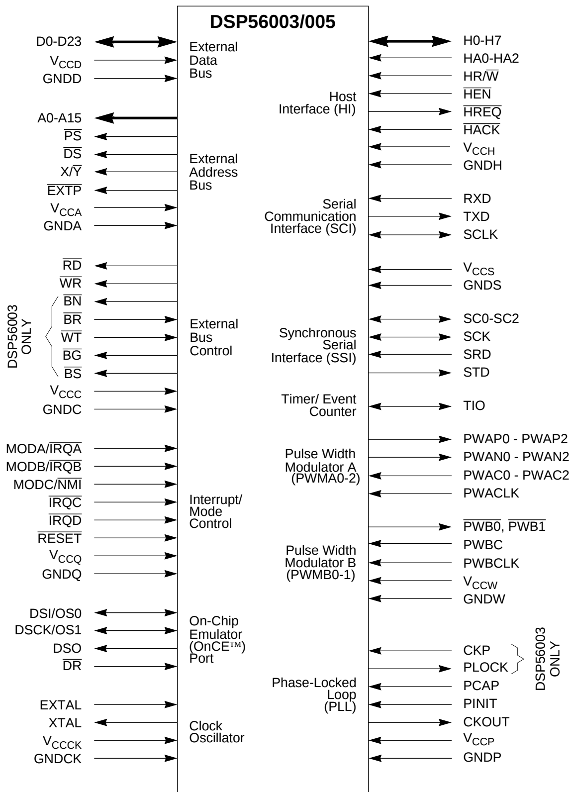
Figure 2-1 DSP56003/005 Signals
