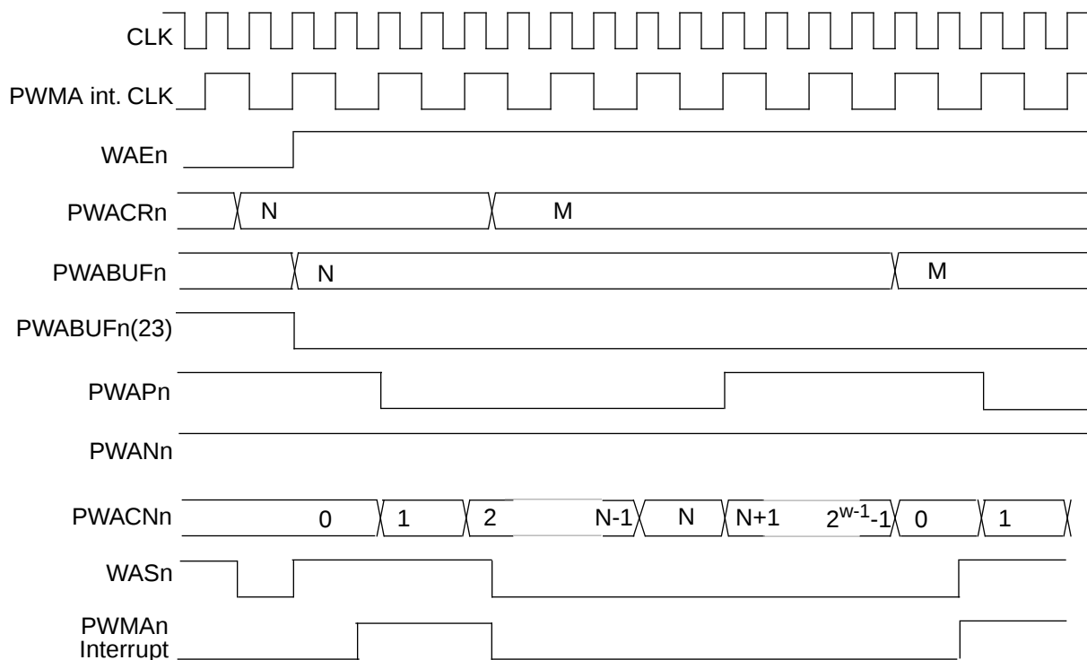
Figure 9-9 PWMA Timing — Internal Clock, Internal Carrier Width=w
