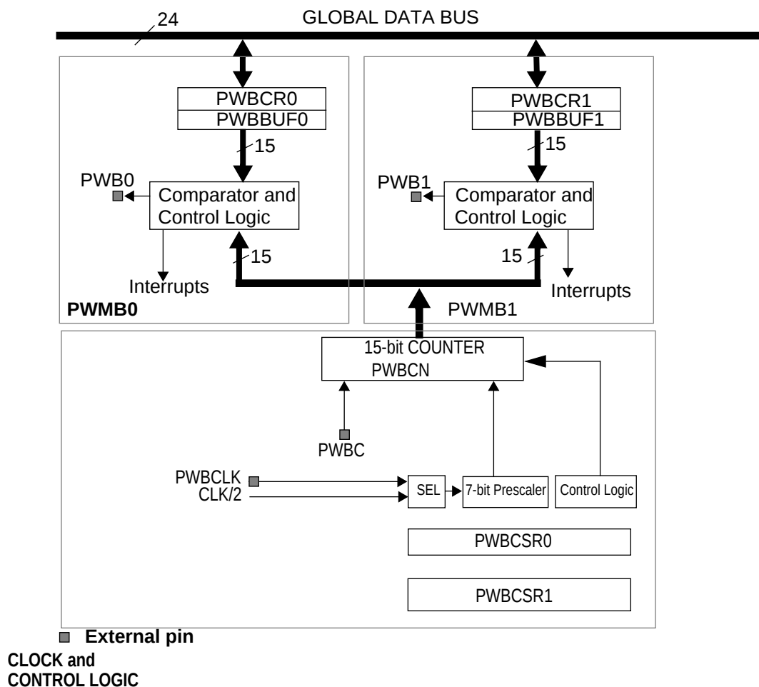
Figure 9-4 PWMB Block Diagram
