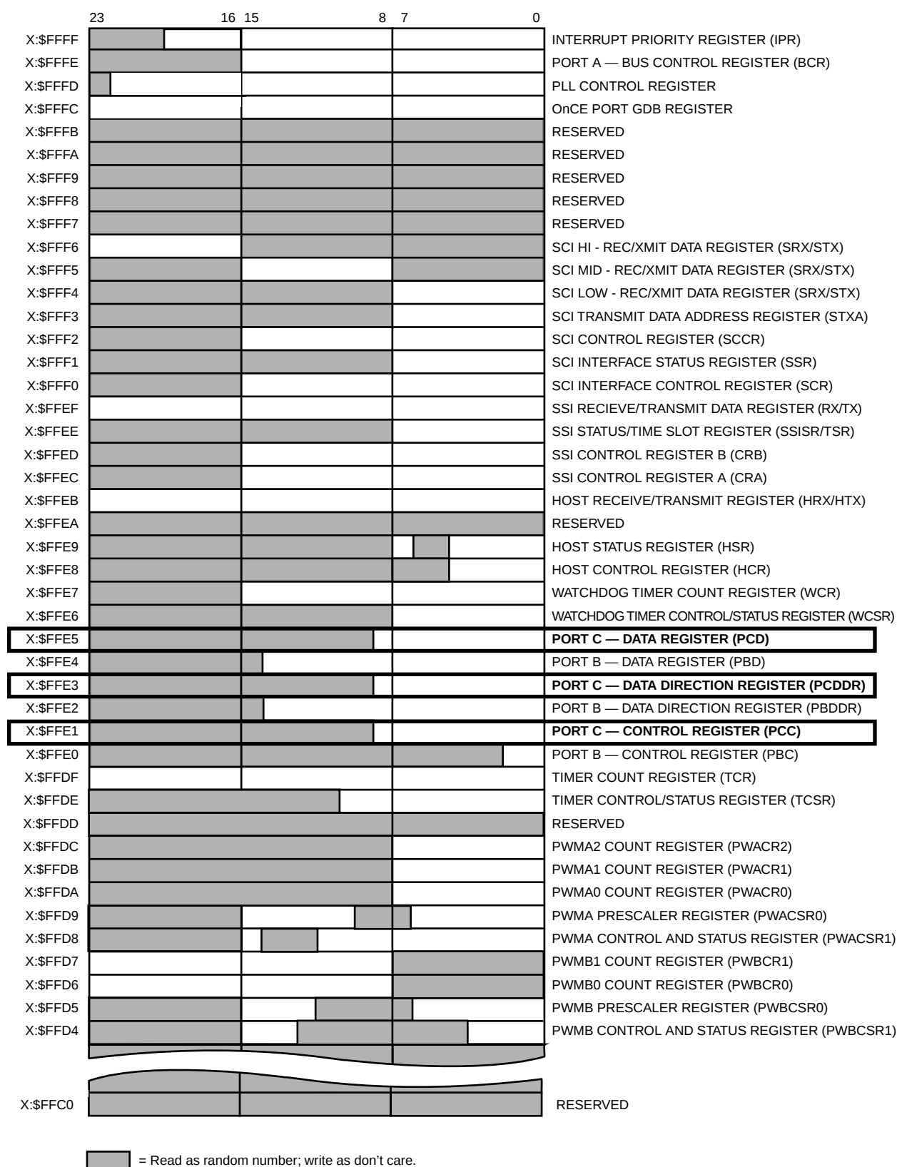
Figure 6-5 On-Chip Peripheral Memory Map
