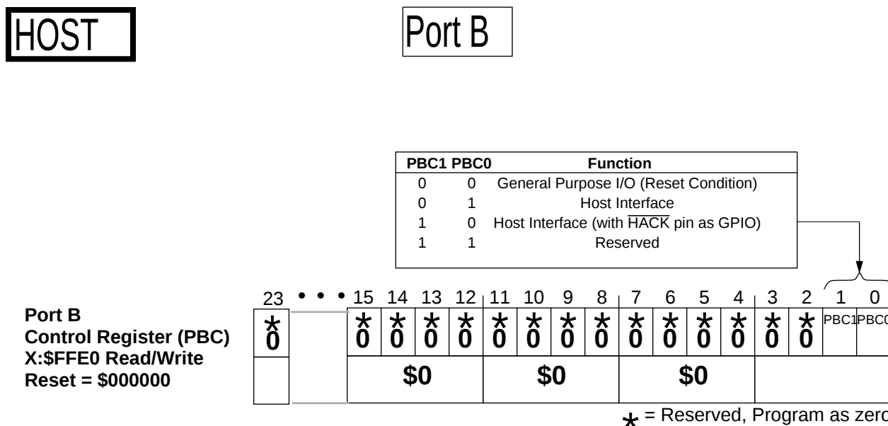
Figure B-13 Port B Control Register (PBC)
