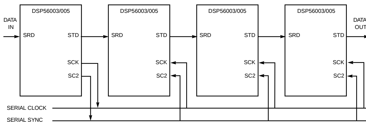
Figure 7-57 SSI Cascaded Multi-DSP System
