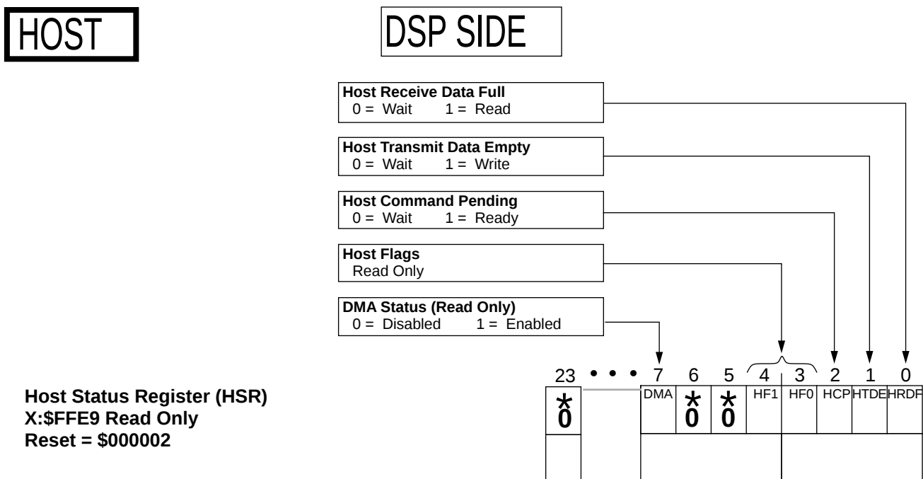
Figure B-15 Host Status Register (HSR)
