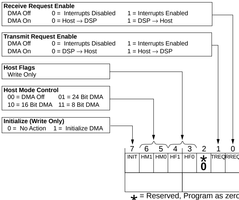
Figure B-18 Interrupt Control Register (ICR)
