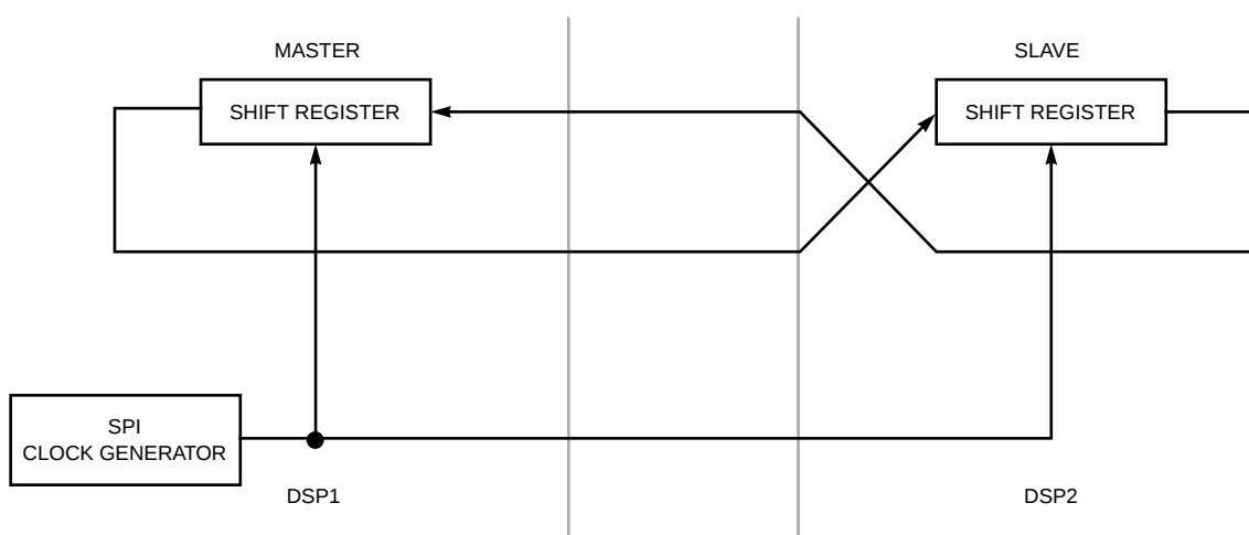
Figure 7-49 SPI Configuration
