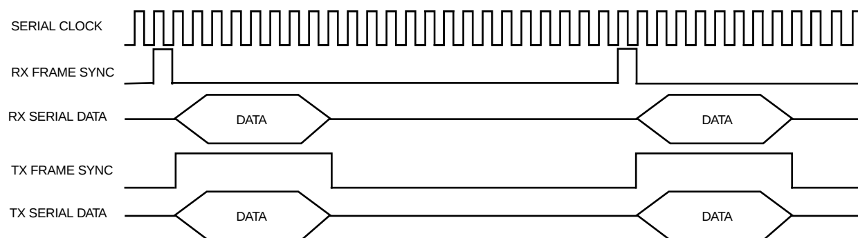
Figure 7-33 CRB FSL0 and FSL1 Bit Operation
