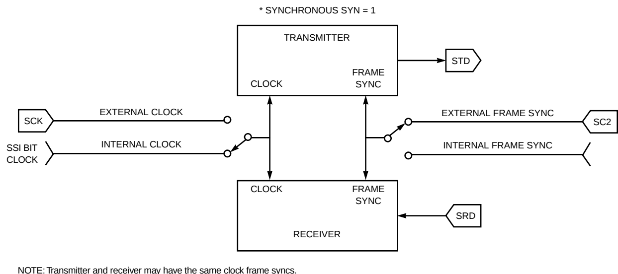
Figure 7-28 CRB SYN Bit Operation
