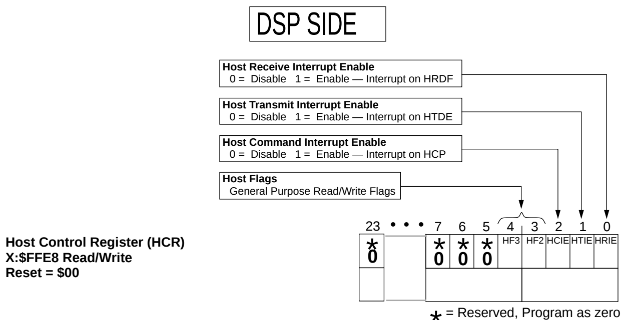
Figure B-14 Host Control Register (HCR)
