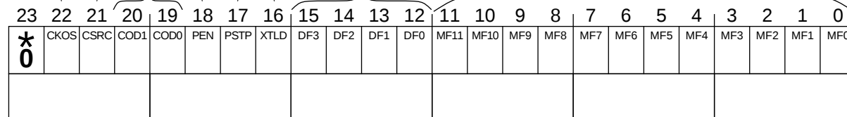
Figure B-6 PLL Control Register (PCTL)
