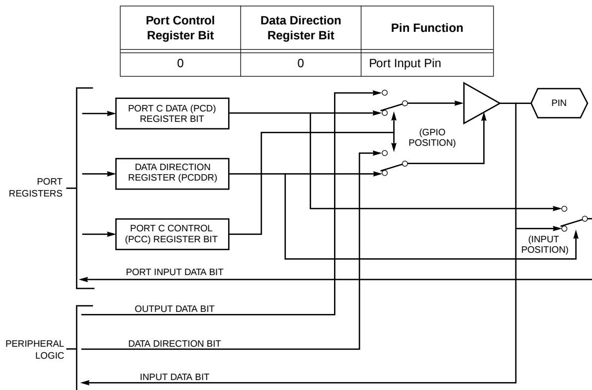
Figure 7-4 Port C I/O Pin Control Logic
