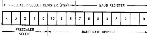
FIGURE 15. UART BAUD Clock Divisor Registers
