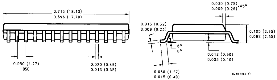
Molded SO Wide Body Package (M) Order Number COP87L84RGM-XE NS Package Number M28B
