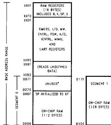
FIGURE 5. RAM Organization
