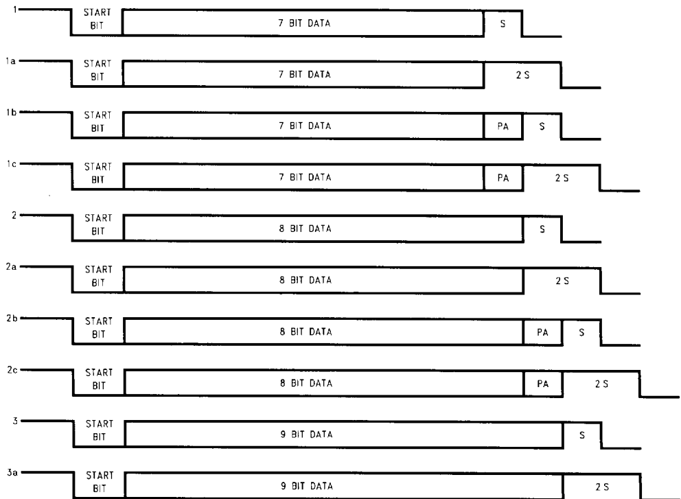
FIGURE 13. Framing Formats
