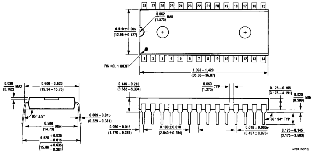
Molded Dual-In-Line Package (N) Order Number COP87L84RGN-XE NS Package Number N28B
