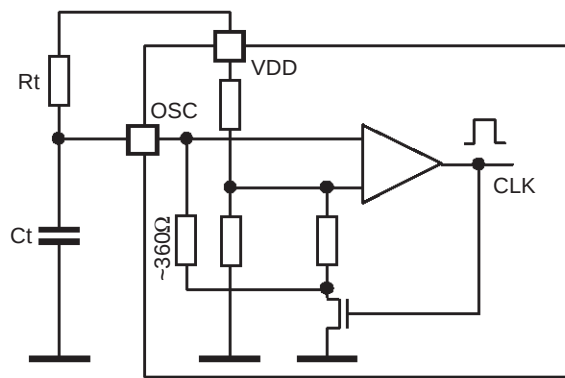
Figure 7: Oscillator
