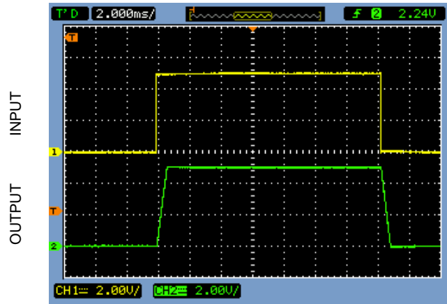
Large-Signal Transient Response V_{DD} = 5.5V , V_{SS} = GND , R_{LOAD} = 100k\Omega , C_{LOAD} = 15pF
