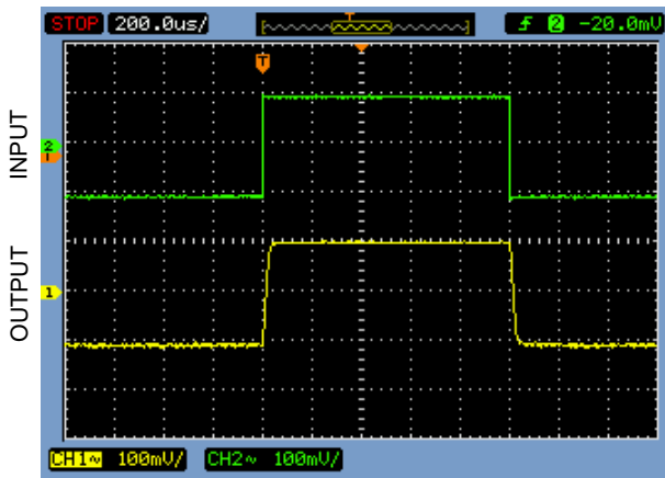
Small-Signal Transient Response V_{DD} = 5.5V , V_{SS} = GND , R_{LOAD} = 100k\Omega , C_{LOAD} = 15pF
