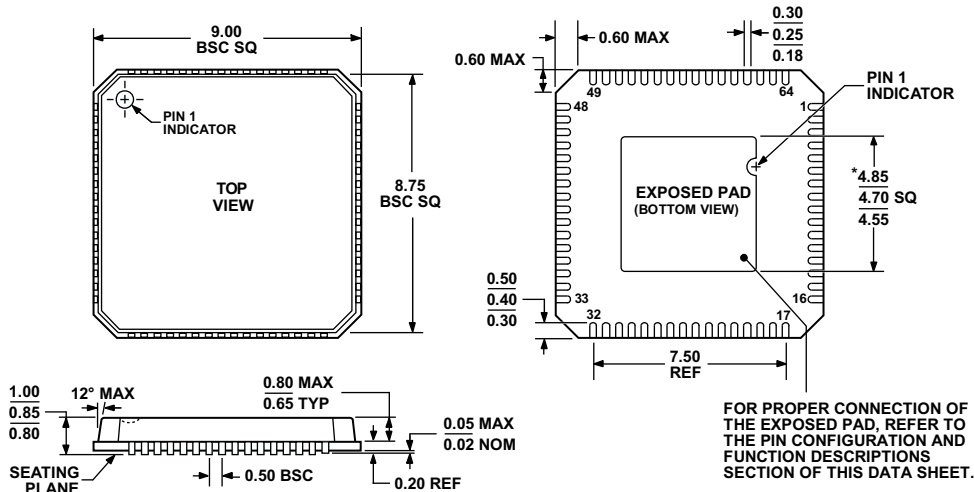
*COMPLIANT TO JEDEC STANDARDS MO-220-VMM4 EXCEPT FOR EXPOSED PAD DIMENSION Figure 6. 64-Lead Lead Frame Chip Scale Package [LFCSP_VQ] 9 mm x 9 mm Body, Very Thin Quad (CP-64-1) Dimensions shown in millimeters
