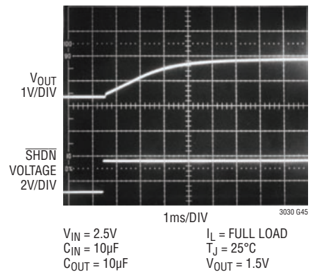
Start-Up Time from Shutdown C_{BYP} = 0.01\mu\text{F}
