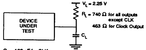
Figure 6: AC TESTING LOADING CIRCUIT
