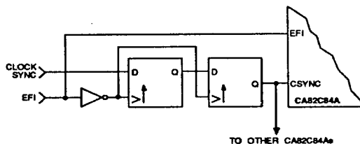
Figure 3 : CSYNC SYNCHRONIZATION
