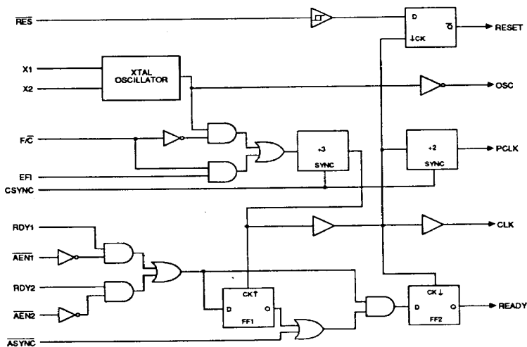
Figure 1 : CA82C84A BLOCK DIAGRAM
