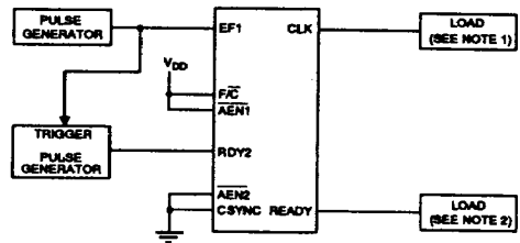
Figure 10: READY TO CLOCK (USING EF1)
