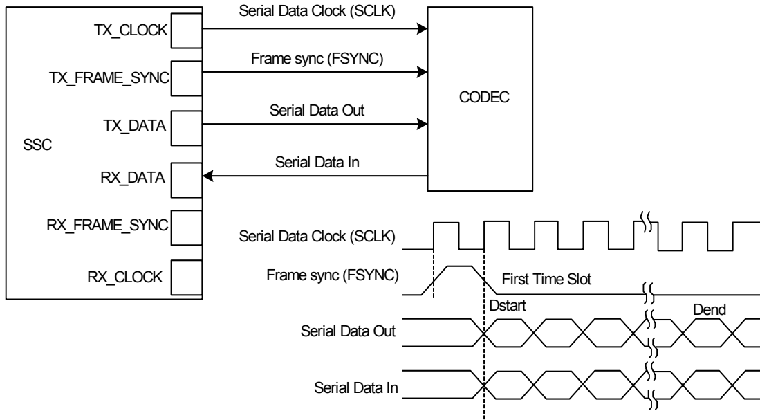
Figure 24-19. Time Slot Application Block Diagram
