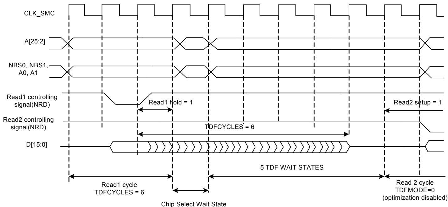
Figure 28-24. TDF Optimization Disabled (MODE.TDFMODE = 0). TDF Wait States between Two Read Accesses on Different Chip Selects.
