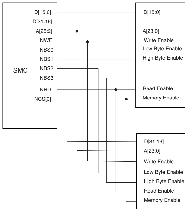
Figure 28-8. Connection of two 16-bit Data Bus on a 32-bit Data Bus: Byte Select Option
