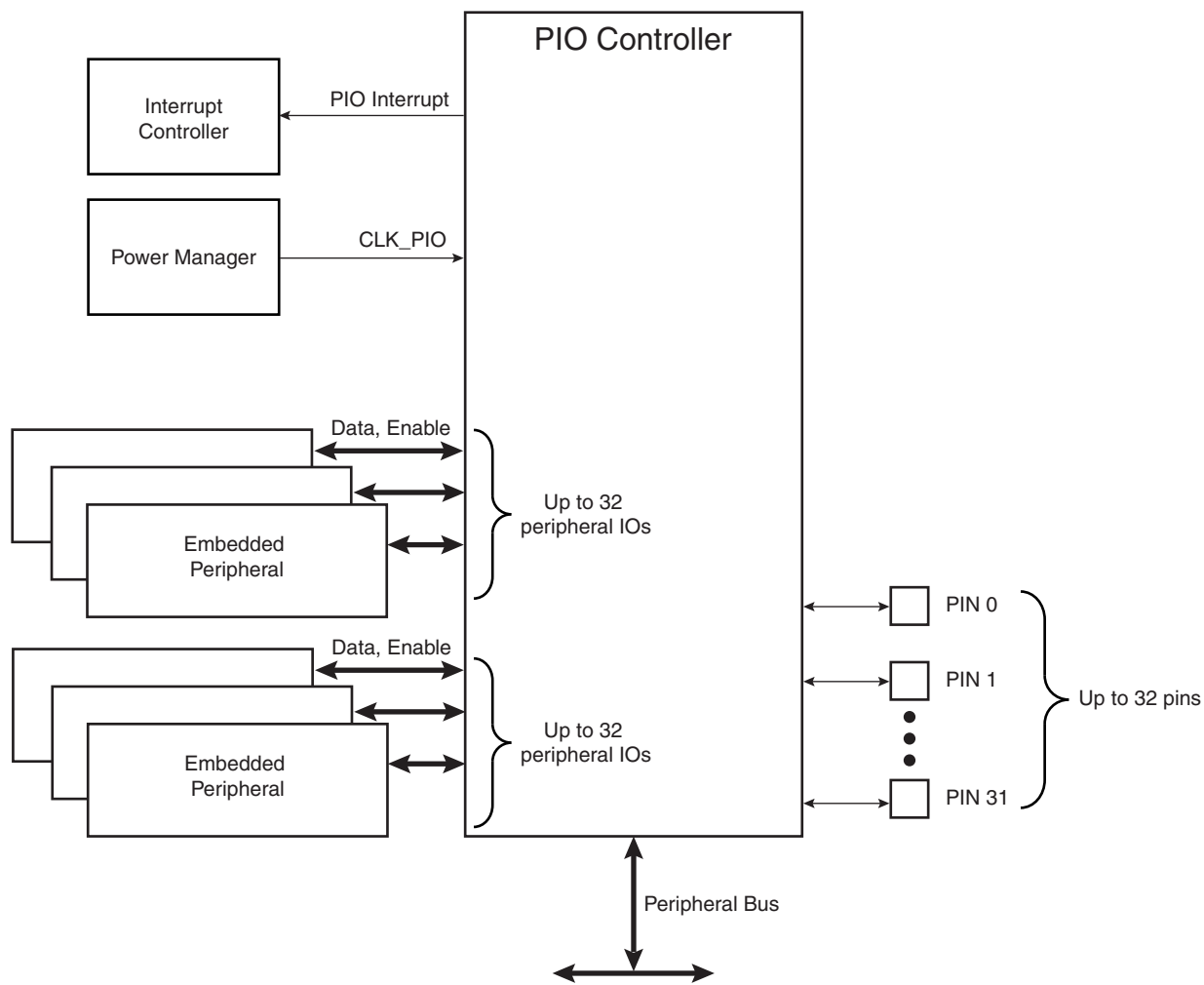
Figure 20-1. Block Diagram
