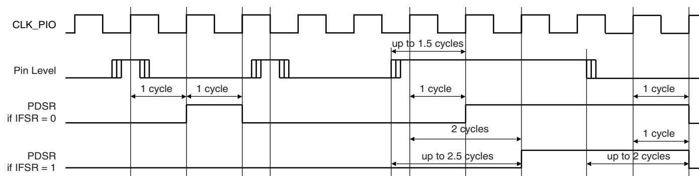
Figure 20-5. Input Glitch Filter Timing
