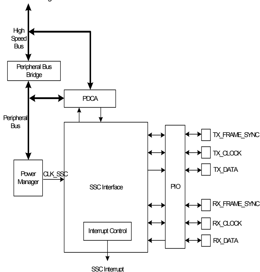
Figure 24-1. Block Diagram
