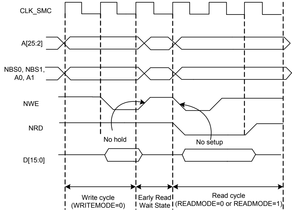
Figure 28-19. Early Read Wait State: NCS Controlled Write with No Hold Followed by a Read with No Setup.
