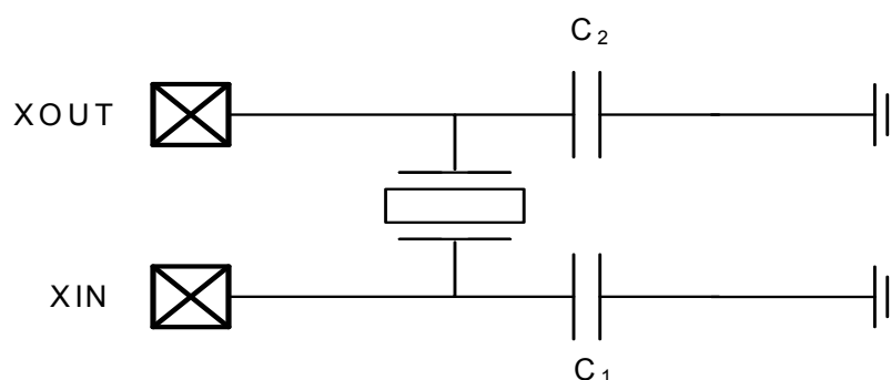
Figure 11-1. Oscillator connections
