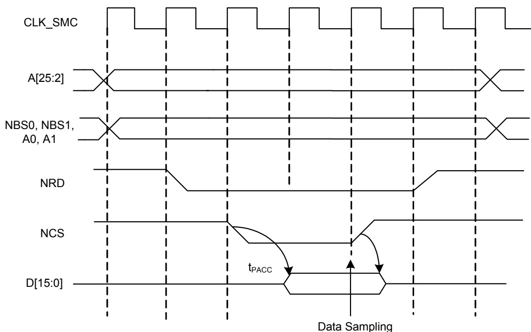
Figure 28-12. READMODE = 0: Data Is Sampled by SMC Before the Rising Edge of NCS
