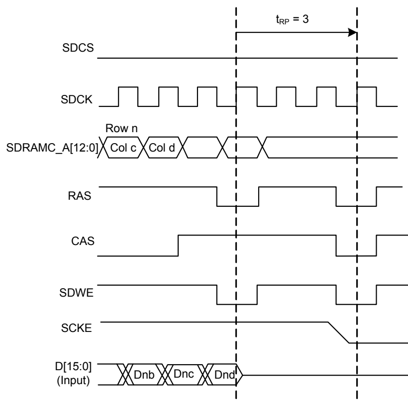
Figure 29-11. Deep Power-down Mode Behavior
