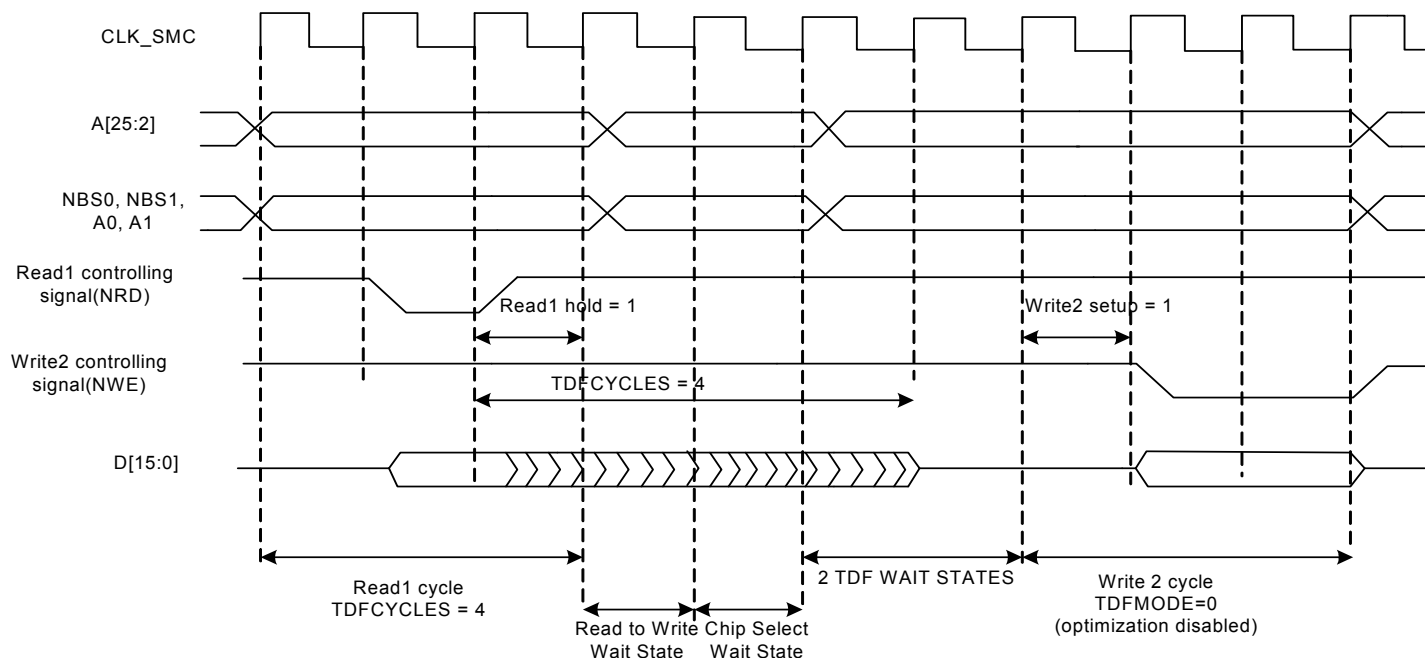
Figure 28-25. TDF Optimization Disabled (MODE.TDFMODE= 0). TDF Wait States between a Read and a Write Access on Different Chip Selects.
