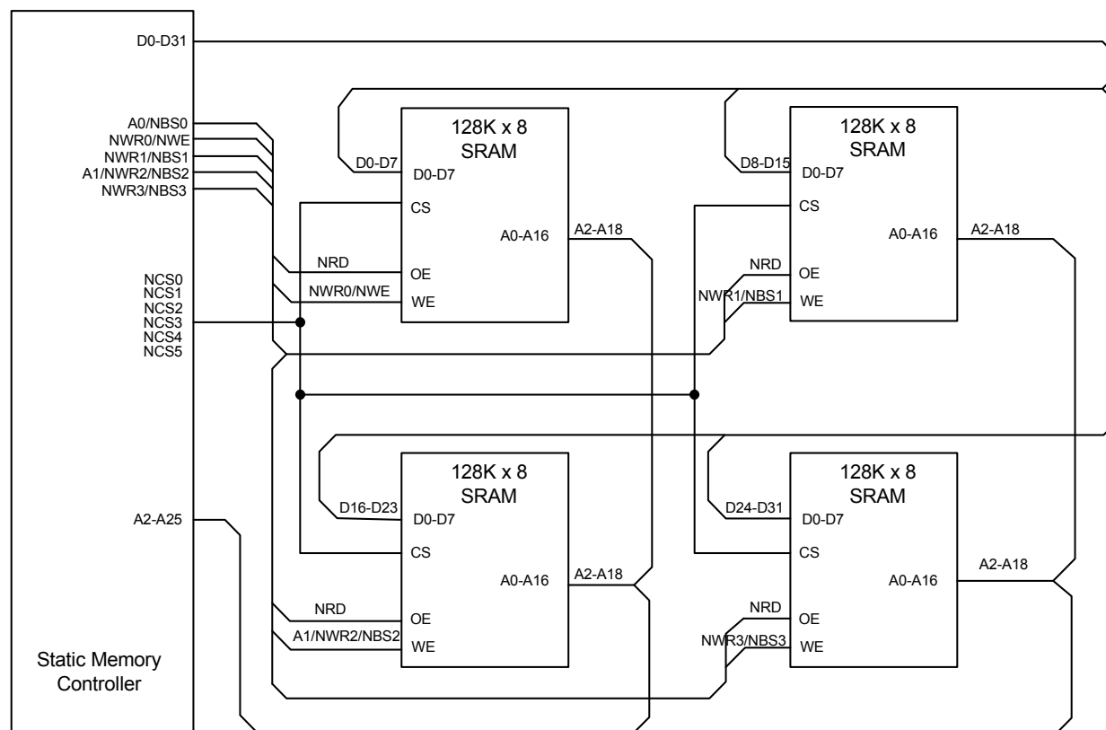
Figure 28-2. SMC Connections to Static Memory Devices
