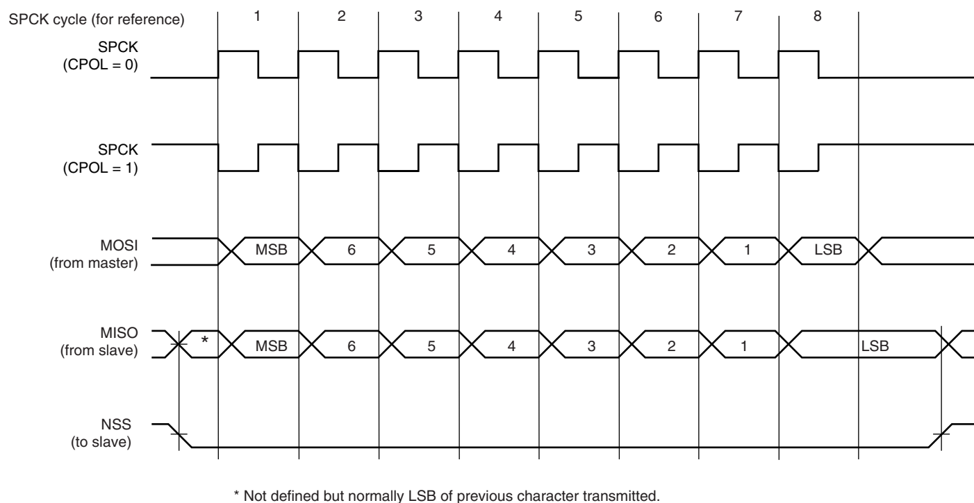
Figure 21-4. SPI Transfer Format (NCPHA = 0, 8 bits per transfer)
