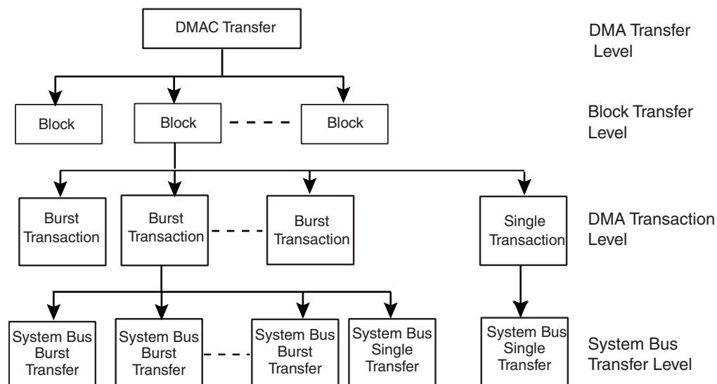
Figure 18-2. DMACA Transfer Hierarchy for Non-Memory Peripheral
