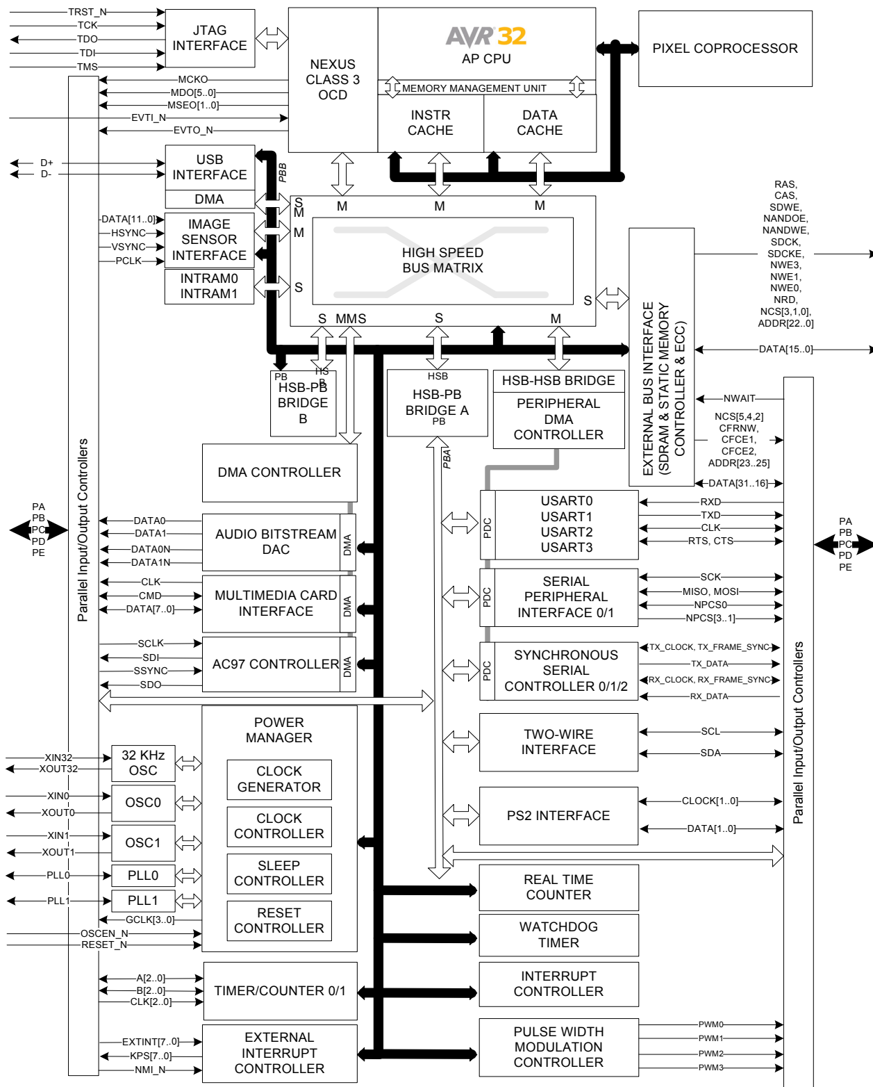
Figure 5-1. Blockdiagram
