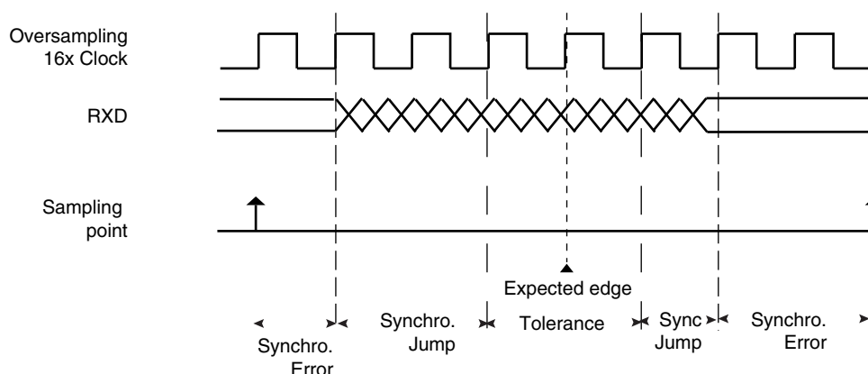
Figure 25-11. Bit Resynchronization
