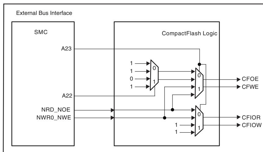
Figure 17-4. CompactFlash Read/Write Control Signals
