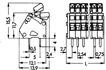
Diameter of drilled holes: 1.1 +0.1 mm L = (No. of poles x 2.54 mm) + 2.3 mm
