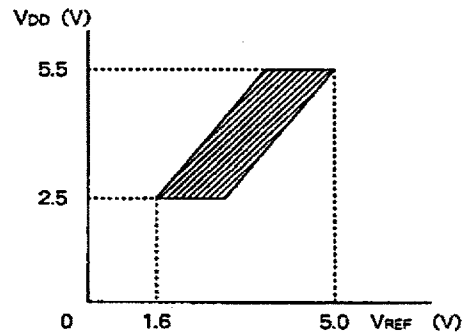
Fig. 5 Power supply voltage detection reset function chart
