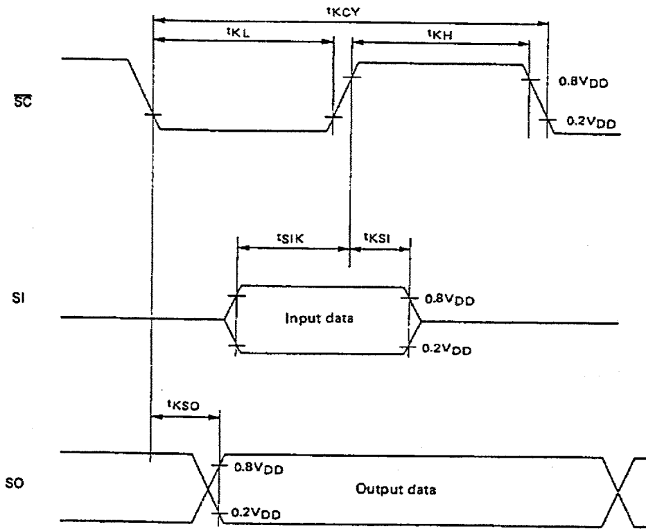
Fig. 4 Serial transfer timing
